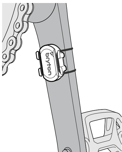
Cadence Sensor
